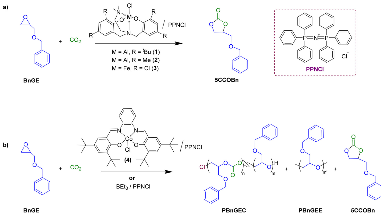
Scheme 1 ROCOP of CO 2 /BnGE catalyzed by (a) {ONNO R2 }MCl/PPNCl (R = t Bu, Me, Cl, M = Al, Fe) complexes resulting in the corresponding five-membered ring benzyloxymethyl cyclic carbonate (5CCOBn), and (b) {Salphen}CoCl/PPNCl or BEt 3 /PPNCl system, resulting in poly(benzyl glycidyl ether carbonate) (PBnGEC), poly(benzyl glycidyl ether) (PBnGEE) and cyclic carbonate (5CCOBn).
