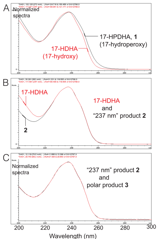
Fig. 3 Overlaid UV spectra from RP-HPLC analysis of 17S-HPDHA autoxidation. Spectra of the starting 17-hydroperoxide 1 and autoxidation products were recorded online in RP-HPLC solvent (CH 3 CN/H 2 O/HAC: 45/55/0.01 by volume, cf. Fig. 2) and are normalized to absorbance maxima. (A) 17-HPDHA and 17-HDHA. (B) 17-HDHA and the “237 nm” product 2 . (C) Spectra of 2 and 3 from RP-HPLC (retention times of ~57 and ~25 min, respectively).
