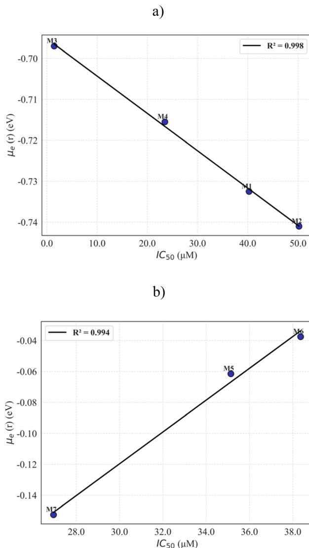
Fig. 8 \mu_e(r) dependence on the experimental IC_{50} values of Bcl-2 using (a) cinnamyls and (b) quinoxalines as inhibitors.
