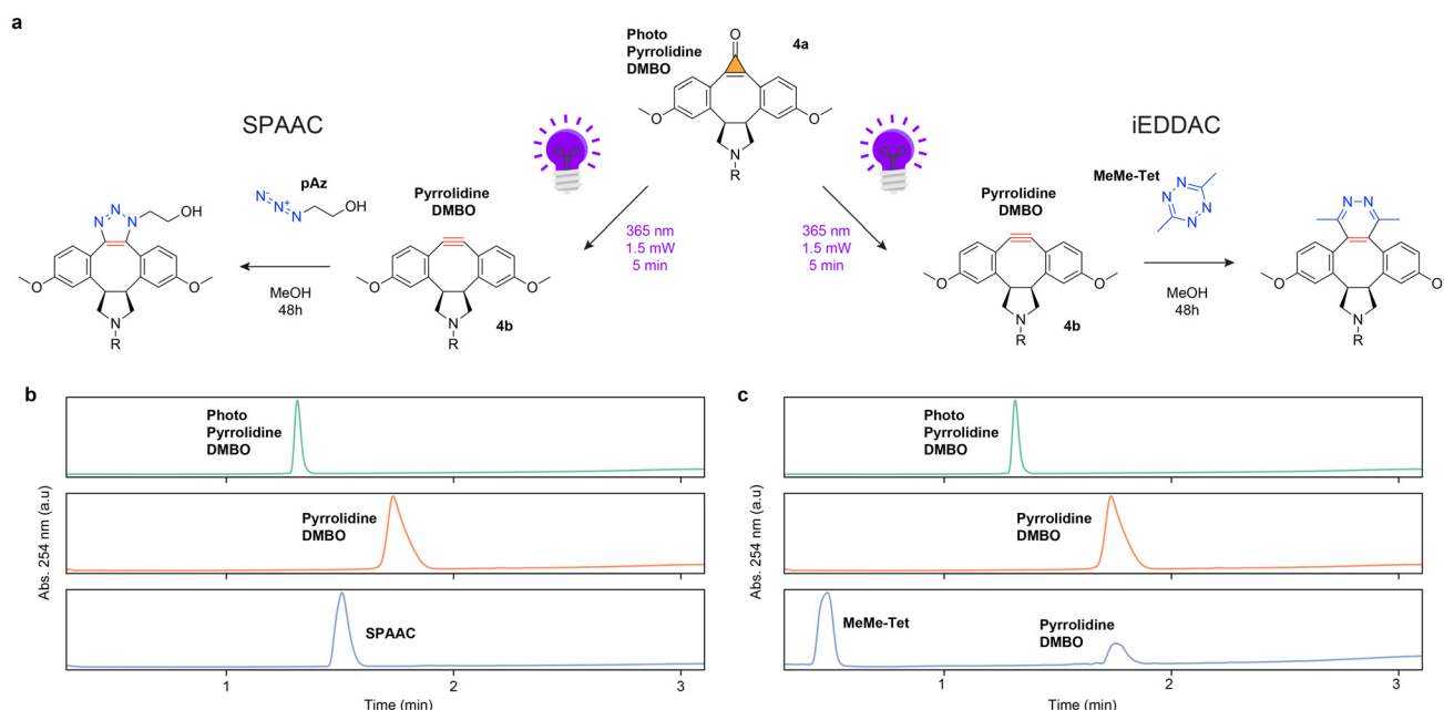
Fig. 2 Pyrrlidine-DMBO reacts with azides but not with tetrazines. (a) Experimental design. Each experimental branch starts out with a pyrrolidine-DMBO with an intact cyclopropanone photocage (photo-pyrrolidine-DMBO). The cyclopropanone cage is decarboxylated by exposure to 1.5 mW of UV light (365 nm wavelength) for 5 minutes resulting in pyrrolidine-DMBO. Lastly either 2-azidoethanol (pAz) or 3,6-dimethyltetrazine (MeMe-Tet) is added and both reactions are allowed to run for 48 hours at room temperature in methanol (MeOH). (b) Liquid-chromatography mass spectrometry (LC-MS) analysis reveals that only pyrrolidine-DMBO shows SPAAC reactivity towards pAz. (c) But no iEDDAC reactivity towards MeMe-Tet; reaction conditions: 250 \mu M cyclooctyne, 2.5 mM pAz or MeMe-Tet, room temperature in methanol, 48 hours.
