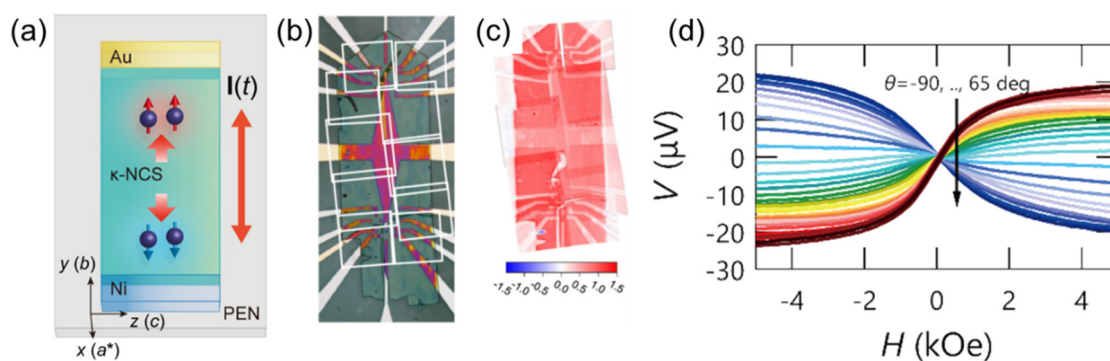
Fig. 7 (a) Schematic of the CISS experiment with \kappa -NCS. AC bias was applied in the b axis direction to drive the spin rectification. (b) Microscopic image of the device. The white squares show the CD microscope fields of view. (c) CD microscopy image of the crystal, which shows a right-handed structure in the entire crystal. The field of view is identical to Fig. 1b. (d) Angle-dependent voltage V across the nickel and gold electrodes. Magnetization M of the nickel electrode was rotated by the external magnetic field H , whose angle to the y axis is defined by \theta .
