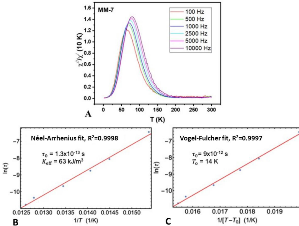
Fig. 7. (A) Representative AC susceptibility \chi''/\chi' versus temperature curves for MM-7, taken at frequencies ranging from 100 Hz to 10,000 Hz. The imaginary part of the magnetic susceptibility is normalized to the real part at 10 K. (B) The logarithm of the peak relaxation time \ln(\tau) versus inverse temperature 1/T with a NA fit through the data (equation (2)). (C) The same data with a Vogel-Fulcher fit (equation (5)) and with the anisotropy constrained to its DC value calculated from the mean diameter of the sample ( K_{\text{eff}}=40 \text{ kJ/m}^3 ).
