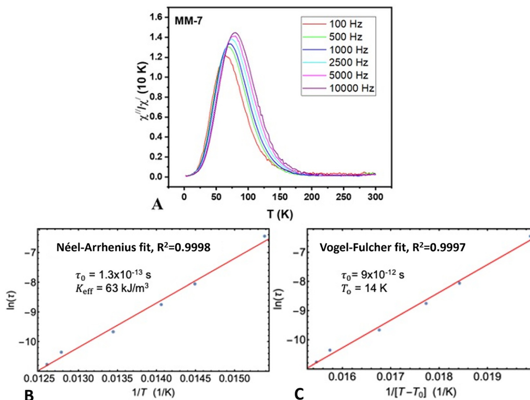
Fig. 7 (A) Representative AC susceptibility \chi''/I\chi' versus temperature curves for MM-7, taken at frequencies ranging from 100 Hz to 10 000 Hz. The imaginary part of the magnetic susceptibility is normalized to the real part at 10 K. (B) The logarithm of the peak relaxation time \ln(\tau) versus inverse temperature 1/T with a NA fit through the data (eqn (2)). (C) The same data with a Vogel–Fulcher fit (eqn (5)) and with the anisotropy constrained to its DC value calculated from the mean diameter of the sample ( K_{\text{eff}} = 40 kJ m -3 ).
