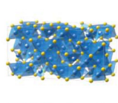
\text{Cu}_3\text{FeS}_4 - bornite
