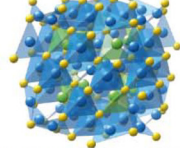
\text{Cu}_{12}\text{Sb}_4\text{S}_{13} - tetrahedrite
