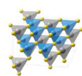
\text{Cu}_2\text{SnS}_3 - mohite
