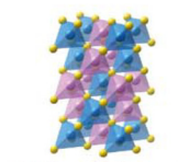
\text{CuFeS}_2 - chalcopyrite
