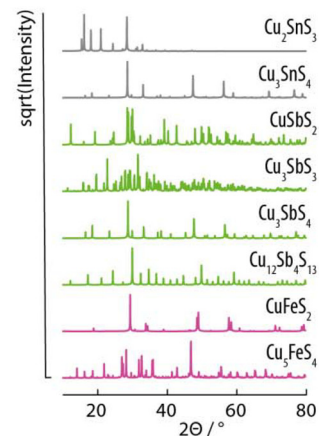
\text{Cu}_{12}\text{Sb}_4\text{S}_{13} - tetrahedrite
