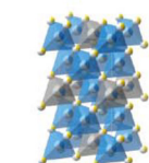
\text{Cu}_3\text{SnS}_4 - kuramite
