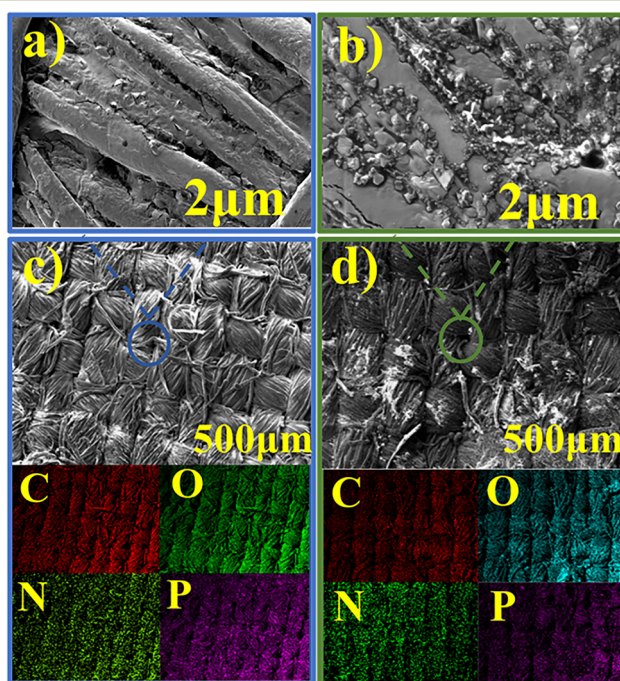
Fig. 5 SEM images and elemental mapping of (a, c) G@PA/PP-coated cotton fabric and (b, d) G@PA/PP-coated cotton fabric after flame test.
