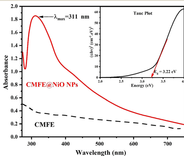
Fig. 1 (a) UV-Vis spectra of CMFE and CMFE@NiO NPs and Tauc's plot of CMFE@NiO NPs (inset).
