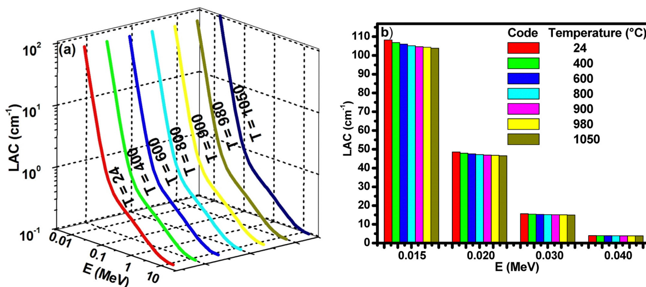
Fig. 3 (a) Three-dimensional surface plot of the LAC for orthoferrosilite as a function of photon energy and temperature. (b) Cross-sections of the surface at four low energies, highlighting the consistent decrease in LAC with increasing temperature across the photoelectric dominance region.
