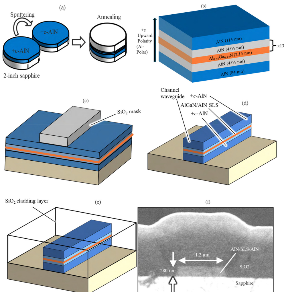
Fig. 5 Fabrication process of TQPM AlN/AlGaN SLS channel waveguide structure. (a) Sputtering and face-to-face annealing of AlN. (b) MOVPE of AlN/AlGaN SLS structure. (c) Formation of \text{SiO}_2 mask. (d) Formation of a channel waveguide by ICP-RIE. (e) Deposition of \text{SiO}_2 cladding layer, dicing, and end-face polishing. (f) Cross-sectional scanning electron microscopic (SEM) image of the fabricated waveguide.
