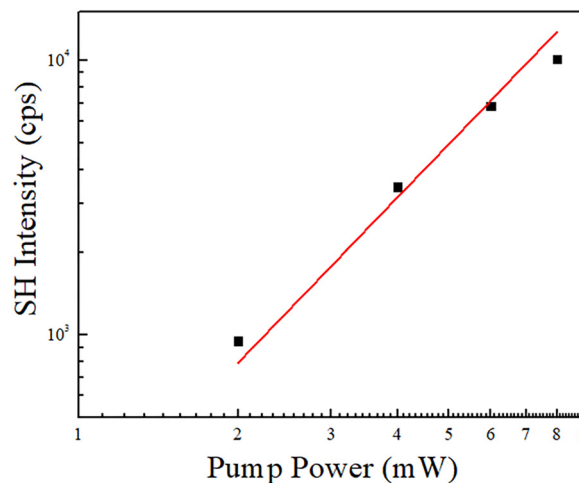
Fig. 8 Dependence of SH intensity on input power.
