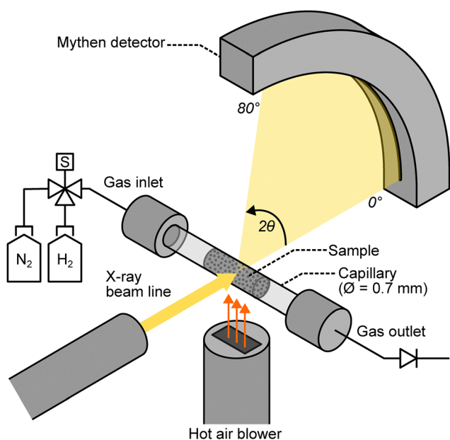
Fig. 2 Schematic of the experimental setup used at ANSTO for synchrotron diffraction measurements of hydrogen reduction at elevated temperature. Photographs of the experimental apparatus are available in Supplementary A.
