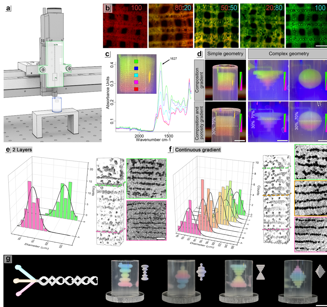
Fig. 2 Operational set-up - (a) schematic representation of 3D printer with the mix-ff chip as printhead; (b) confocal images of 3D printed grids of mixed compositions of DexMA:GelMA at various mixing ratios: 100 : 0, 80 : 20, 50 : 50, 20 : 80, 0 : 100, reporting the efficiency of the mixing; (c) FTIR spectra at specific points of DexMA:GelMA gradient samples; (d) 3D printed porous structures inside the agarose fluid-gel bath that were printed using two different fluorescent dyes in the continuous phases (the first line exhibits a graded transition between two colors, indicating a compositional gradient between two materials along the z-axis. In the second line, while the compositional gradient remains consistent with the first line, a density gradient is introduced. This density variation is evident in the fluorescence intensity of the dyes: regions with a stronger fluorescence signal correspond to higher density (low porosity), whereas regions with a weaker fluorescence signal indicate lower density (high porosity)); (e) and (f) Micro-CT analysis of porous FGMs. Three-dimensional reconstruction of the scaffold obtained from X-ray image stacks and a representative horizontal cross-section (right), together with the corresponding pore size distribution (left). (g) Schematic representation of 3 inlets micromixer and 3D printed complex geometries with gradient composition evidenced by smooth gradient of color. Scale bars: (b) 1 mm, (d) 5 mm (e) 1 mm (f) 500 \mu\text{m} (g) 1 mm.
