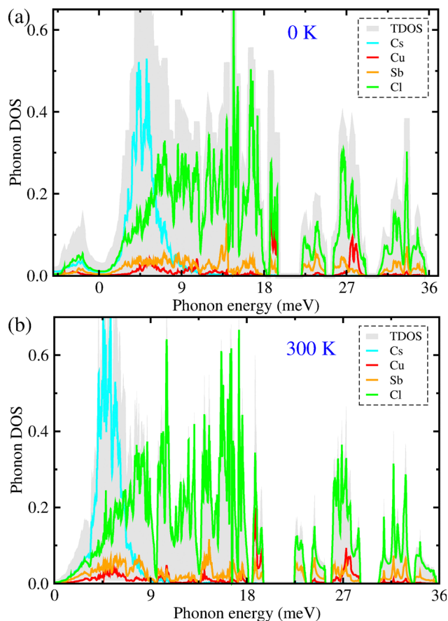
Fig. 3 Atom-resolved phonon density of states (DOS) calculated at (a) 0 and (b) 300 K by the self-consistent phonon (SCP) theory for the quadruple halide perovskite \text{Cs}_4\text{CuSb}_2\text{Cl}_{12} with the monoclinic phase of the C2/m space group.
