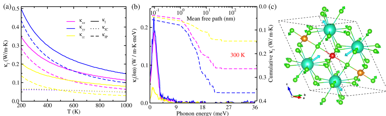
Fig. 5 (a) Lattice thermal conductivity \kappa_l (solid) with Peierls's contribution \kappa_{lP} (dashed) and coherent contribution \kappa_{lC} (dotted) as functions of temperature T , (b) thermal conductivity spectra \kappa_l(h\omega) as a function of phonon energy (solid) and cumulative \kappa_l as a function of mean free path (dashed) calculated on top of the SCP eigenvalues at 300 K, and (c) ball-and-stick view of rattling vibrations of constituent atoms corresponding to the lowest optical phonon mode at the \Gamma point of the phonon BZ for the quadruple halide perovskite \text{Cs}_4\text{CuSb}_2\text{Cl}_{12} with the monoclinic phase of the C2/m space group. The cyan, red, orange and green balls (arrows) represent the Cs, Cu, Sb and Cl atoms (atomic vibration), respectively.
