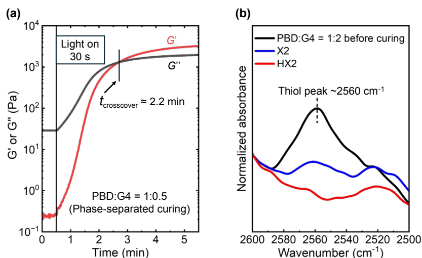
Figure 1: (a) Photo-rheological analysis of the phase-separated X0.5 resin (PBD:G4 = 1:0.5) formulation under UV irradiation (i.e., 10 mW/cm 2 ), showing the evolution of G' and G'' over time; (b) ATR-FTIR spectra of the original photoresin (PBD:G4 = 1:2) before curing (black) and cured X2 (blue) and HX2 (red) samples.
