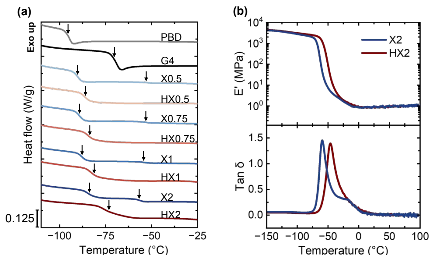
Figure 3: (a) DSC thermograms of neat PBD, neat G4, and photocured PBD–G4 samples with (X0.5–X2) and without (HX0.5–HX2) macroscopic phase separation at varying compositions; (b) DMA temperature sweeps of X2 and HX2: E' vs. T (top) and \tan \delta vs. T (bottom). The arrows in (a) denote T_g s determined by DSC.
