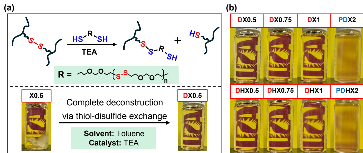
Figure 5: (a) Reaction scheme and decrosslinking experiment showing the deconstruction of thiol-ene PBD–G4 networks through dynamic thiol-disulfide exchange reactions; (b) Decrosslinking results for photocured PBD–G4 samples with (X0.5–X2) and without (HX0.5–HX2) macroscopic phase separation at varying compositions. D represents complete network deconstruction, while PD represents partial network deconstruction.
