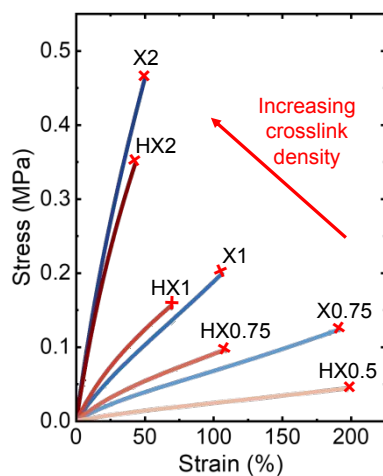
Figure 4: Room-temperature tensile test results for photocured PBD-G4 samples with (X0.75–X2) and without (HX0.5–HX2) macroscopic phase separation at varying compositions. Note that the X0.5 film was sticky and not self-standing, thus not suitable for tensile testing.
