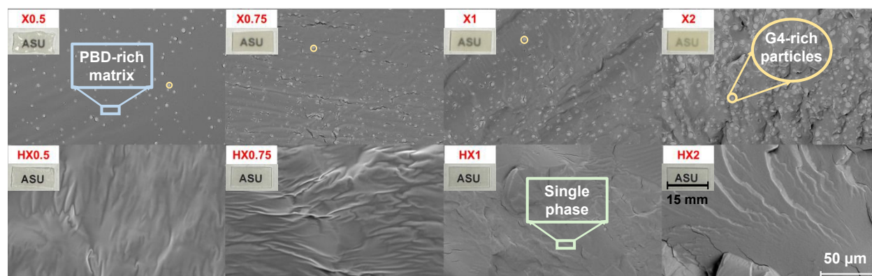
Figure 2: Representative digital photographs and SEM images for photocured PBD–G4 samples at varying compositions, with (X0.5–X2) vs. without (HX0.5–HX2) macroscopic phase separation. (Areas marked with yellow circles are G4-rich dispersed domains and areas marked with blue boxes are PBD-rich matrix, respectively; Areas marked with green boxes are the mixed single phase comprising both PBD and G4.)
