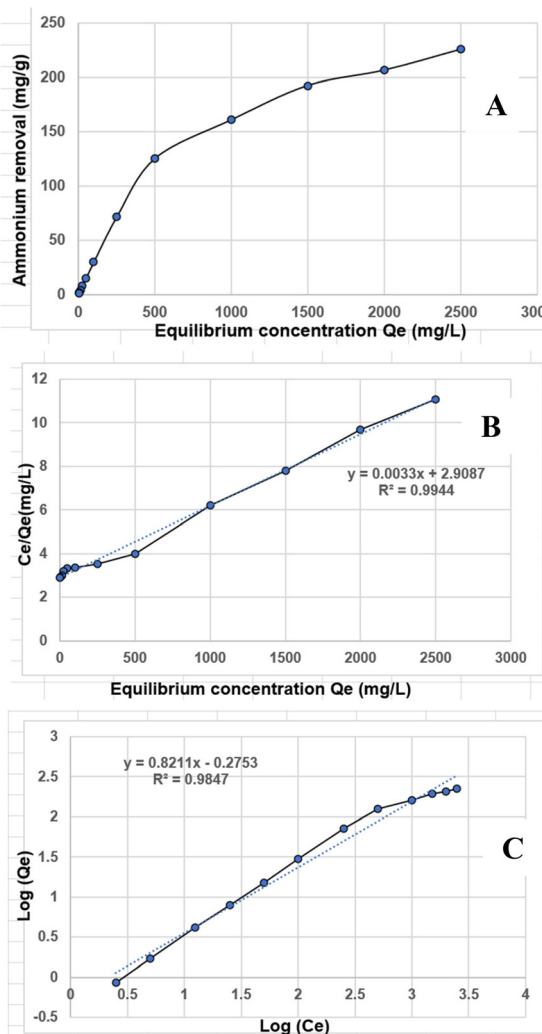
Fig. 5 (A) Relationship between \text{NH}_4^+ removal and equilibrium concentration; (B) Langmuir isotherm for \text{NH}_4^+ removal using CNFs; (C) Freundlich isotherm for \text{NH}_4^+ removal using CNFs.
