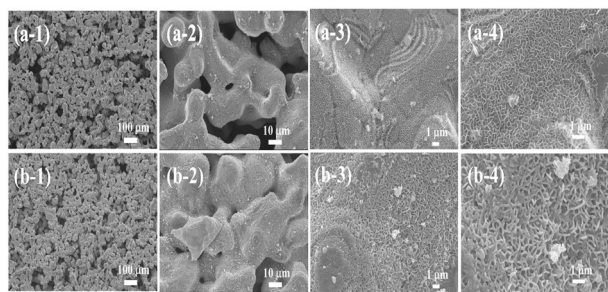
Fig. 2 SEM images of (a-1)–(a-4): NiFe foam at magnifications of 100 \times , 1000 \times , 5000 \times , and 10 000 \times , respectively; (b-1)–(b-4): NiMo@NiFe foam at magnifications of 100 \times , 1000 \times , 5000 \times , and 10 000 \times , respectively.
