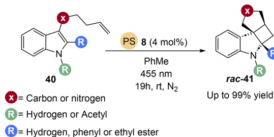
Fig. 9 Dearomative photocyclization catalyzed by 8 .
