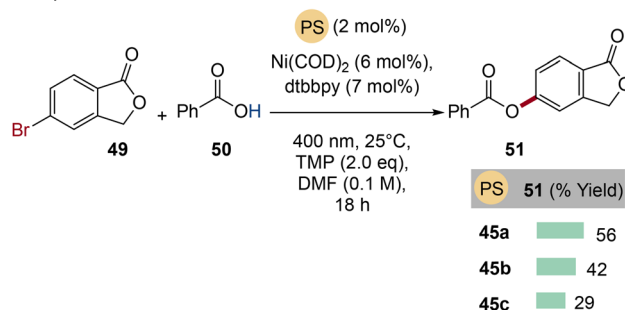
Fig. 11 Reactivity of 45 derivatives in representative examples.
