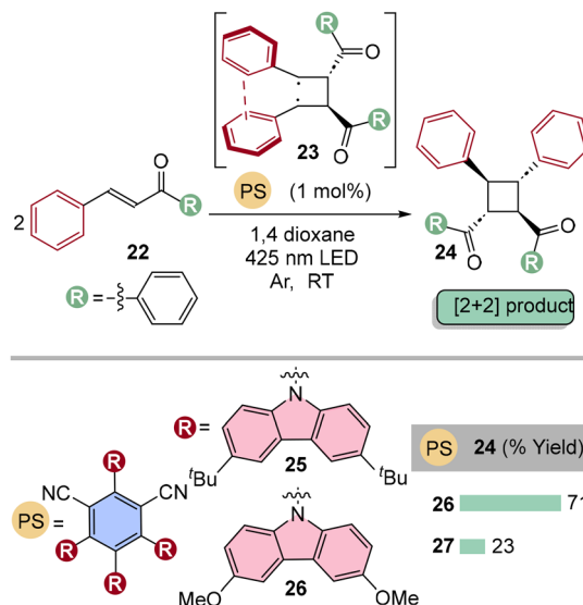
Fig. 5 Comparison of the activity of the photosensitizers 25 and 26 for the synthesis of compound 24 .
