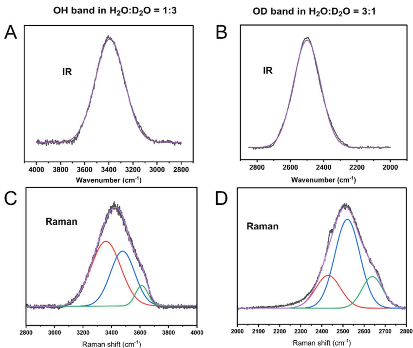
Fig. 1 ATR-IR (A and B) and Raman (C and D) spectra of bulk 1 M KOH in 1 : 3 H 2 O : D 2 O (A and C) and 3 : 1 H 2 O : D 2 O (B and D) showing the O–H (A and C) and O–D (B and D) stretching bands of HOD. In (A) and (B), the black traces correspond to the experimental ATR-IR spectra and the purple line to the corresponding Gaussian fit. The spectrum of the Si–air interface was used as the background in (A) and (B). In (C) and (D), the black traces correspond to the experimental Raman spectra and the red, blue and green lines correspond to the corresponding deconvolution into three Gaussian components. The purple trace corresponds to the sum of those three components.
