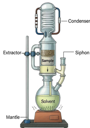
Fig. 4 The Soxhlet apparatus used for lipid extraction.
