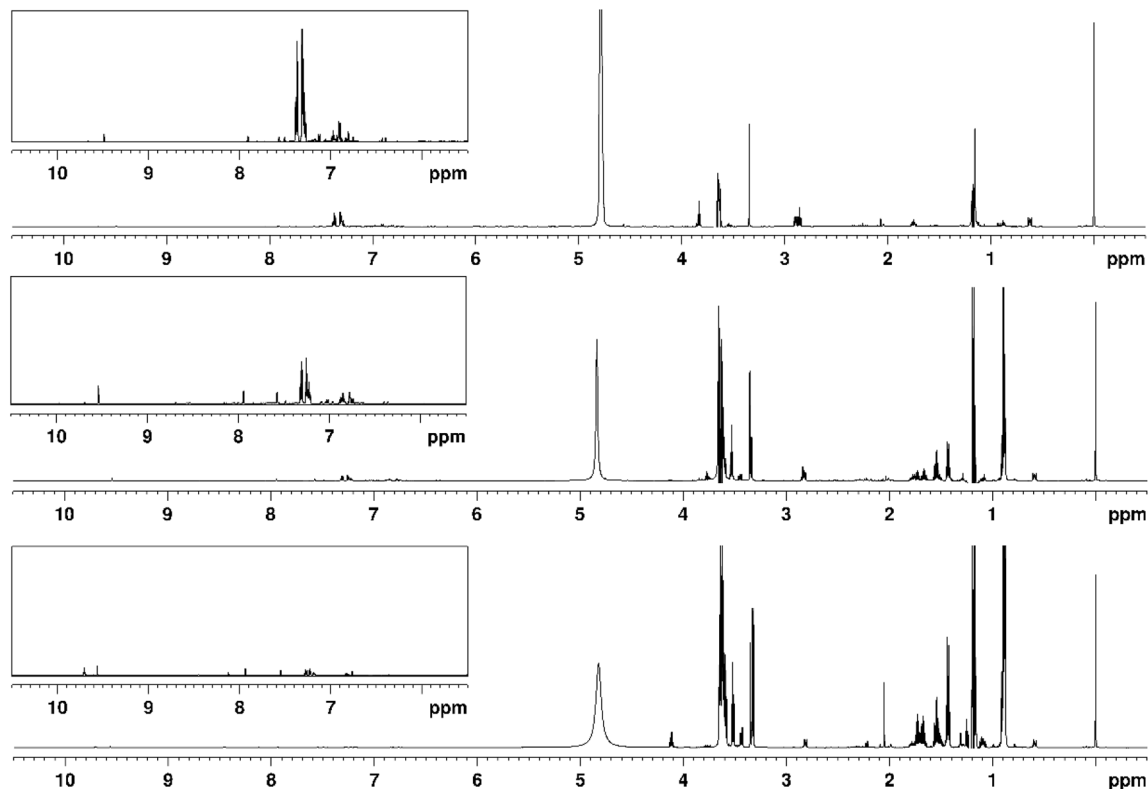
Fig. 6 ^1\text{H} NMR spectra of peated spirit distillation fractions 1, 2 and 3 (from bottom to top), recorded at 600 MHz.
