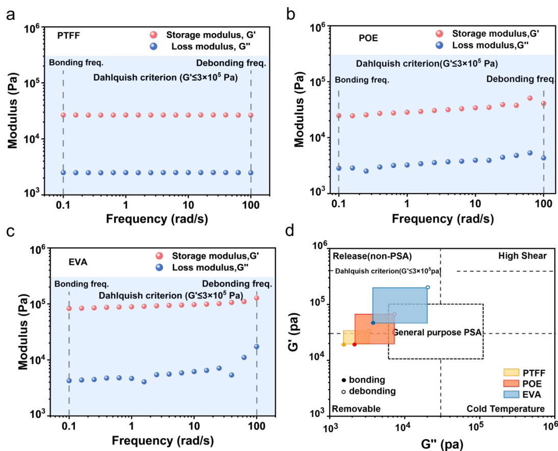
Fig. 5. Analysis of polymer applications based on viscoelastic window. G' and G'' of (a) PTFE, (b) POE and (c) EVA obtained from frequency dependent DMA (25 °C, \gamma=0.1\% ). (d) The corresponding viscoelastic window analysis of PTFE, POE and EVA.
