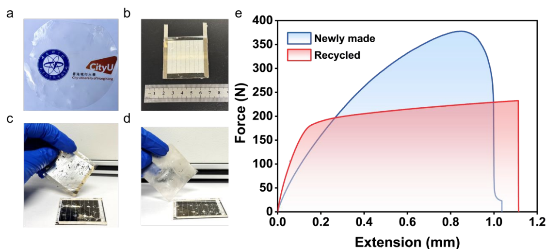
Fig. 7 Evaluation of the Recyclable Performance of PTFE. (a) Original PTFE encapsulation film. (b) Electrode side display of PSC module encapsulated based on PTFE lamination technology. (c)
