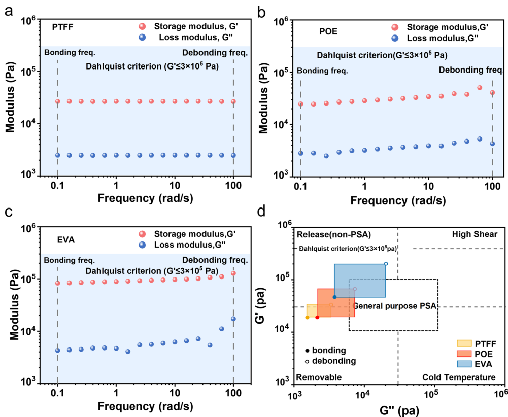
Fig. 5 Analysis of polymer applications based on viscoelastic window. G' and G'' of (a) PTFE, (b) POE and (c) EVA obtained from frequency dependent DMA ( 25 ^{\circ} C, \gamma = 0.1\% ). (d) The corresponding viscoelastic window analysis of PTFE, POE and EVA.
