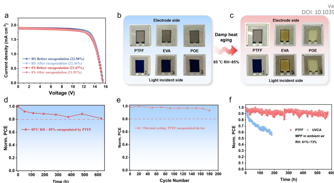
Fig. 6 The impact of encapsulation on device performance. (a) Performance of the PSC module before and after encapsulation by PTFF. (b) Devices encapsulated by PTFF, EVA, and POE before damp-heat aging. (c) Devices after damp-heat aging in (b). (d) The performance of the PTFF encapsulated device during the damp heat aging test. (e) Performance of the PTFF encapsulated device in thermal cycling aging test. (f) MPP tracking of devices encapsulated by different materials.
