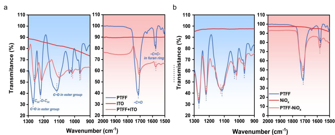
Fig. 3 Interaction between PTFF and substrates at the contact surface evidenced by FTIR. (a) FTIR spectra of PTFF, ITO and their mixture. (b) FTIR spectra of PTFF, \text{NiO}_x and their mixture.
