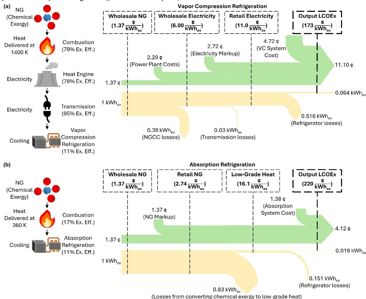
Fig. 5. LCOEx Sankey diagrams for (a) vapor compression and (b) absorption refrigeration. Both systems use natural gas (NG) as the primary energy source, but the process of converting the chemical exergy within NG to high-grade heat, which is used to produce electricity and drive vapor compression refrigeration is significantly more exergetically efficient than using NG to produce low-grade heat and drive absorption refrigeration. This leads to cost benefits for vapor compression refrigeration.
