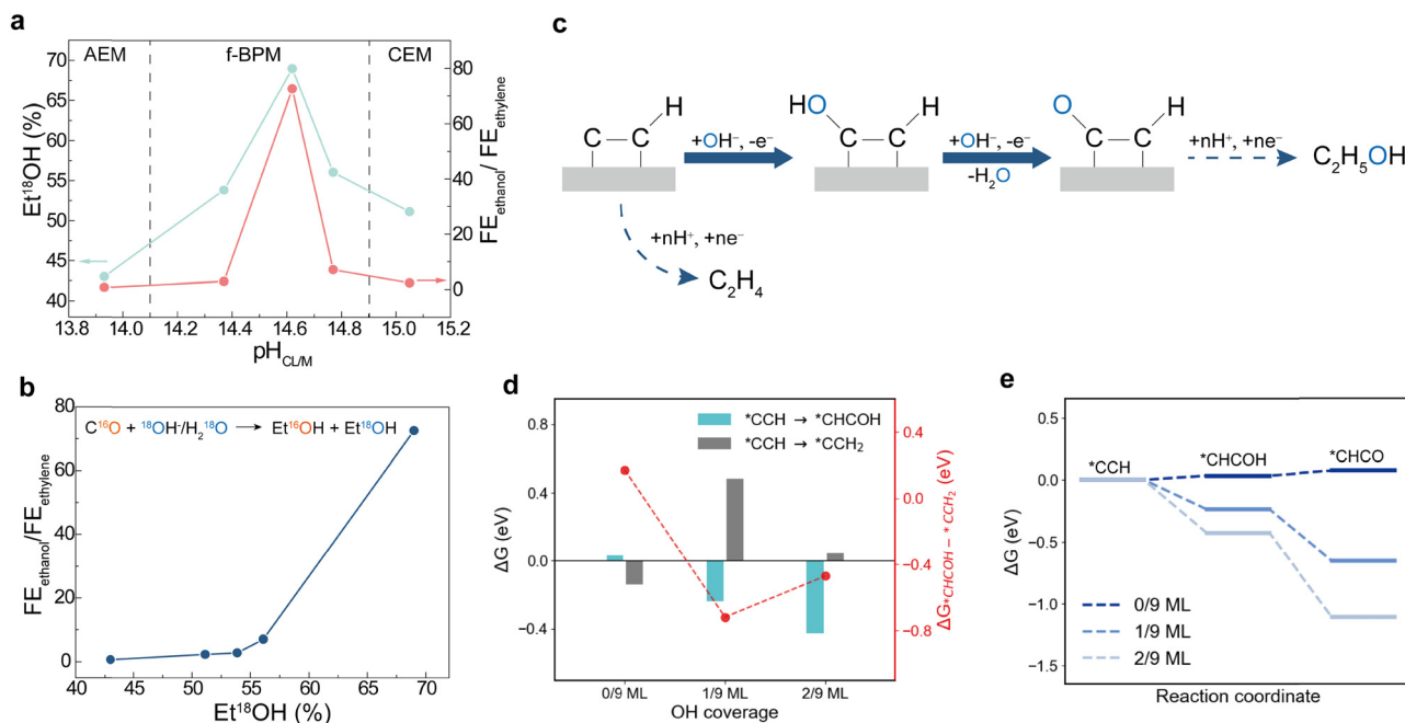
Fig. 4 EC-MS isotope analysis and proposed mechanism. (a) Ethanol/ethylene selectivity and 18 O-ethanol percentage as functions of membrane type (corresponding \text{pH}_{\text{CL/M}} ) in the MEA setup. (b) Ethanol/ethylene selectivity versus 18 O-ethanol percentage in the MEA setup. (c) Key reaction pathways for the CO reduction reaction (CORR) to ethanol on Cu(111). (d) The reaction energies for the ^*\text{CCH} \rightarrow ^*\text{CHC}^{18}\text{OH} and ^*\text{CCH} \rightarrow ^*\text{CCH}_2 steps (left axis) and their corresponding energy differences (right axis, \Delta G_{^*\text{CHCOH} \rightarrow ^*\text{CCH}_2} ) at -0.4 V vs. SHE at various OH coverages. \Delta G_{^*\text{CHCOH} \rightarrow ^*\text{CCH}_2} represents the relative preference for ^*\text{CHCOH} or \text{CCH}_2 formation, where a higher \Delta G_{^*\text{CHCOH} \rightarrow ^*\text{CCH}_2} value indicates more favorable ^*\text{CHCOH} formation and consequently higher ethanol selectivity. (e) Calculated Gibbs free-energy diagram for ^*\text{CCH} to ^*\text{CHCO} on Cu(111) at -0.4 V vs. SHE at various OH coverages.
