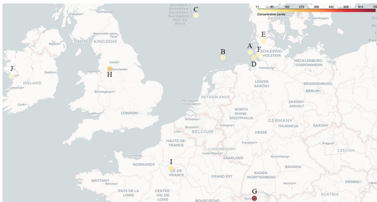
Figure 6 Atmospheric concentrations of 8:2 FTOH ( \text{pg}/\text{m}^3 ) in selected regions in Europe, as reported in prior studies 61,83–87 . Measurements in the following locations are reported: A: German Bight, B: Heligoland, C: West Frisian coast, D: Cuxhaven, E: Schleswig-Holstein, F: Büsum, G: Zurich, H: Manchester, I: Paris, J: Mace Head.
