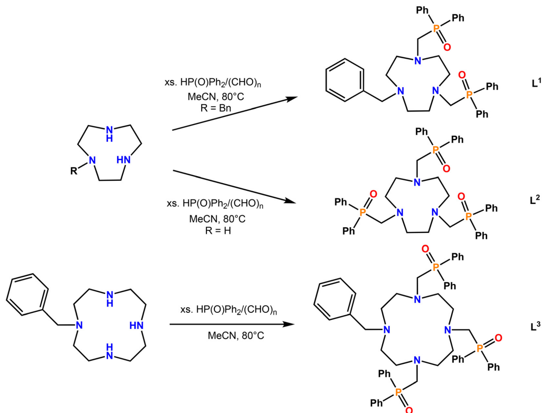
Scheme 2 Synthesis routes used to prepare \text{L}^1 – \text{L}^3 .
