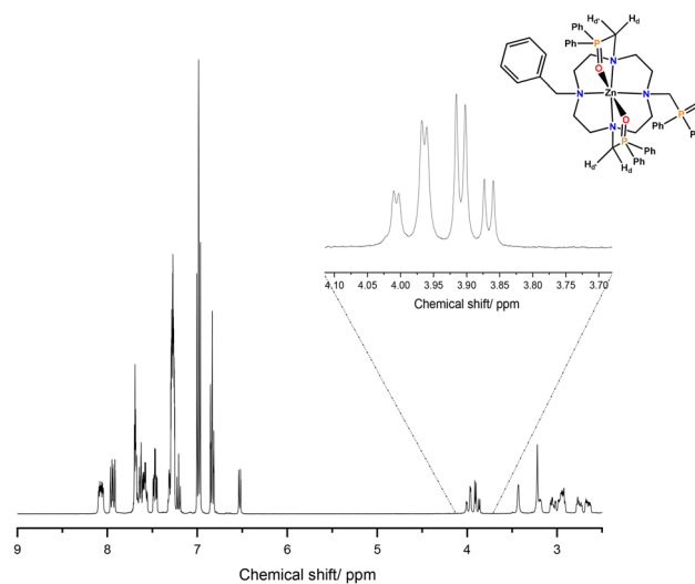
Fig. 5 ^1\text{H} NMR spectrum of [\text{Zn}(\text{L}^3)](\text{BPh}_4)_2 in \text{CD}_3\text{CN} . The expansion (top right) shows the resonance from the diastereotopic methylene protons from the coordinated phosphine oxide arms.
