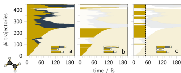
Fig. 3 Comparison of three trajectory-filtering strategies applied to a trajectory ensemble of ethene (A01; taken from ref. 35 and 36). Filtering is performed sequentially using two criteria: (i) a maximum allowed change in potential energy between consecutive frames in the active state of \Delta E_{\text{pot}}^{\text{active}} \leq 0.7 eV; and (ii) a maximum C–H bond length of 250 pm. Each trajectory is represented by a horizontal bar; the vertical ordering is arbitrary. Segments removed by the energetic filter are shown in pale yellow, those removed by subsequent geometric filtering in white, and segments retained for the final analysis are shown in yellow. (a) Both criteria are applied by truncation, yielding trajectories that are first cut by the energy threshold (blue) and then further truncated on the basis of the geometric threshold (yellow). (b) The energy criterion is applied by truncation, whereas the geometric criterion is applied by omission, so that trajectories exceeding the C–H threshold at any time are removed entirely (white). (c) Both criteria are applied by truncation, followed by a transection at 50 fs (black dashed line), which removes all trajectories shorter than this time and cuts the remaining ones accordingly.
