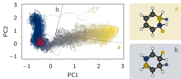
Fig. 6 PCA biplot for the SH data of 1,3-cyclohexadiene (R02). (Left) PCA representation of R02 (ref. 36 and 52) showing the projection onto the first two principal components. Data points are color-coded by the distance between the two sp^3 carbon atoms that are cleaved during the photoinduced electrocyclic 6\pi ring-opening reaction. (Right) Representative molecular structures highlighting atom pairs associated with the dominant PCA loadings (a and b). Loading (a) corresponds to the primary reaction coordinate and captures the C–C bond breaking accompanied by a coupled change in the C–H distance, defined between one of the cleaving sp^3 carbon atoms and a hydrogen atom bound to the opposite cleaving carbon. Loading (b) is dominated by distances between the hydrogen atoms attached to the sp^3 carbons and the central sp^2 carbons, indicating an out-of-plane ring distortion (puckering). The plot was generated using the data of R02 reported as shnitse1-tools datatree on Zenodo. 37
