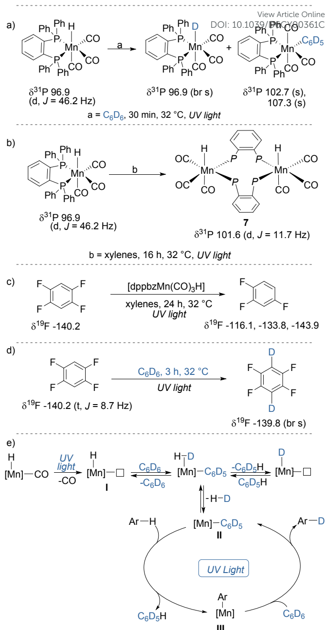
Scheme 5 a) Manganese speciation in the presence of UV light and C 6 D 6 ; b) Self-reaction of [dppbzMn(CO) 3 H]; c) Defluorination of 1,2,4,5-tetrafluorobenzene by [dppbzMn(CO) 3 H] in the absence of C 6 D 6 ; d) C–H HIE of 1,2,4,5-tetrafluorobenzene by [dppbzMn(CO) 3 H] in the presence of C 6 D 6 ; e) Proposed catalytic cycle for the (hetero)arene C–H HIE catalysed by [dppbzMn(CO) 3 H].
