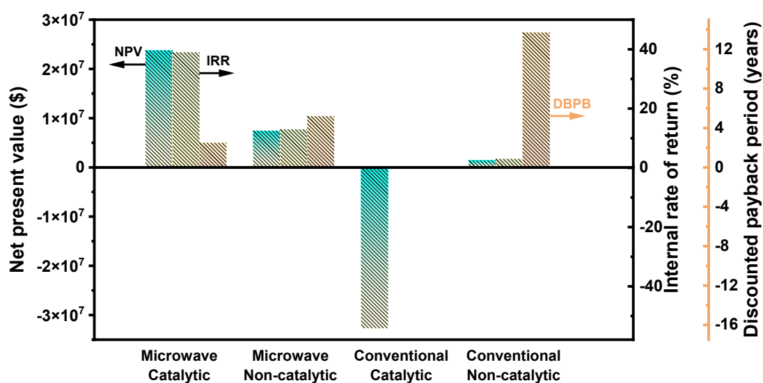
Fig. 7 The techno-economic assessment of microwave catalytic pyrolysis of plastic waste to hydrogen and carbon nanotube.
