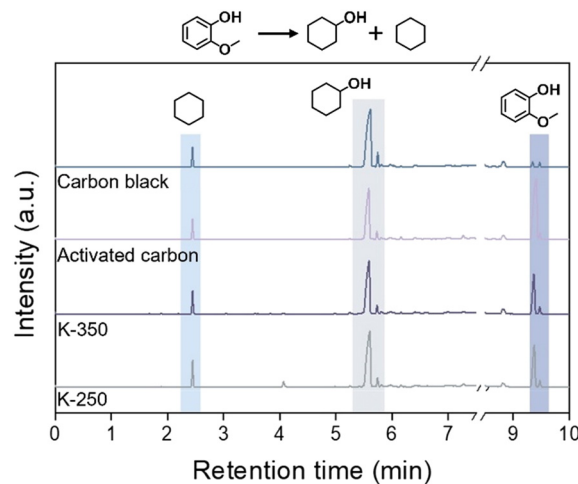
Fig. 9 GC-MS results of Ru catalysts supported on carbon black, activated carbon, K-350, and K-250.
