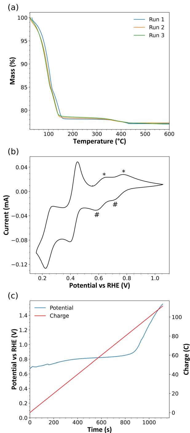
Fig. 3 a) Triplicate TGA data for \text{H}_3[\text{PMo}_{12}\text{O}_{40}]\cdot x\text{H}_2\text{O} , b) cyclic voltammogram of PMA collected at 10\text{ mV s}^{-1} indicating the reduction (#) and oxidation (*) peaks associated with redox cycling of this material in aqueous solution, c) a plot of operating potential ( versus RHE) and charge passed as a function of time during re-oxidation of a reduced PMA solution, showing sustained hydrogen generation at <0.85\text{ V vs. RHE} due to POM-mediated electrolysis before rising sharply when fully discharged.
