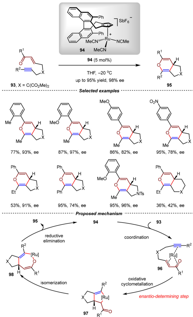
Scheme 24 Ruthenium (II)-catalyzed asymmetric intramolecular [4+2] cycloadditions of yne-enones.
