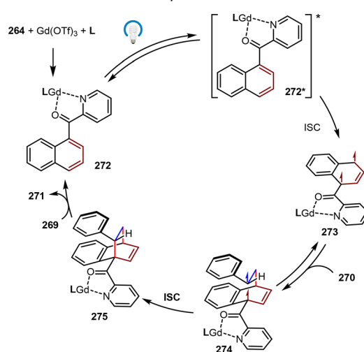
Scheme 54 Gd(III)-catalyzed asymmetric [4+2] photocycloadditions of naphthalenes and styrenes.
