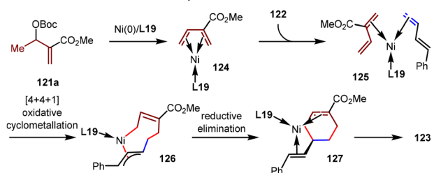
Scheme 28 Ni(0)-catalyzed [4+2] cycloadditions of Morita-Baylis-Hillman carbonates with 1,3-dienes.
