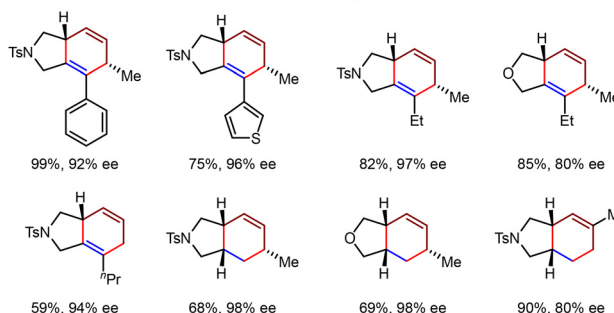
Scheme 31 \text{Co}(\text{I}) -catalyzed intramolecular [4+2] cycloaddition reactions of unactivated diene-ynes and trienes.
