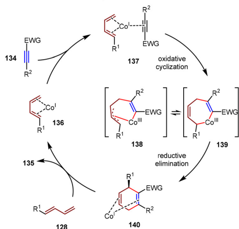
Scheme 30 \text{Co}(\text{I})/\text{BenzP}^* -catalyzed asymmetric [4+2] cycloadditions of 1,3-dienes and alkynes.
