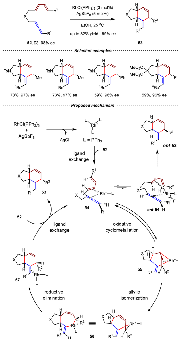
Scheme 16 Rh(PPh 3 ) 3 SbF 6 -catalyzed intramolecular [4+2] cycloadditions of optical active allene-1,3-dienes.
