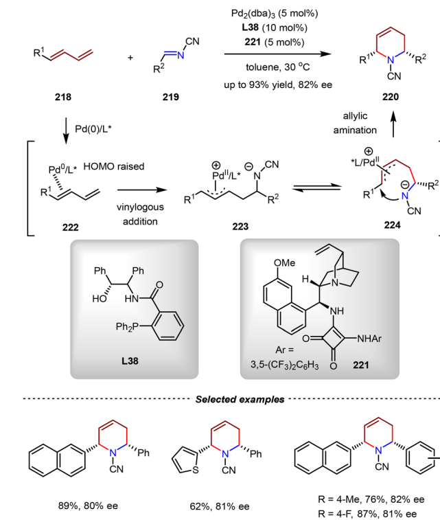
Scheme 46 Pd(0)-catalyzed asymmetric aza-[4+2] cycloadditions of acyclic 1,3-dienes with N -cyano imines.
