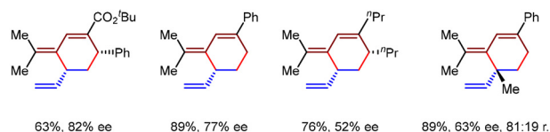
Scheme 21 Pd(0)-catalyzed asymmetric intermolecular [4+2] cycloadditions of vinylallenes and 1,3-dienes.
