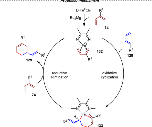
Scheme 29 Fe(I)/ \alpha -diimine-catalyzed asymmetric cross-[4+2] cycloadditions of unactivated 1,3-dienes.
