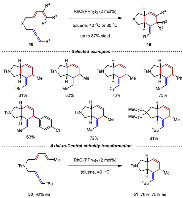
Scheme 15 RhCl(PPh 3 ) 3 -catalyzed intramolecular [4+2] cycloadditions of 1,3-disubstituted allene-1,3-dienes.
