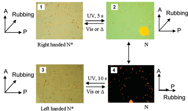
Fig. 16 Photo-responsive systems enabling selective reflection tuning of LC materials. Polarized optical photomicrographs of a planar aligned film based on a cyclic azobenzenophane at room temperature, showing reversible phase transitions occurring by light irradiation of the sample inside a 5 \mu\text{m} cell. 120 Reproduced with permission. 120 Copyright © 2010 American Chemical Society.
