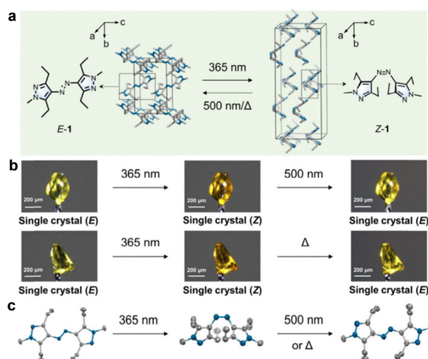
Fig. 3 Photo-responsive systems enabling single crystal-to-single crystal conversion. (a) SCSC E \rightleftharpoons Z isomerization. (b) Photographs of single crystals with reversible SCSC isomerization. (c) Related X-ray molecular structures. 90 Reproduced with permission. 90 Copyright © 2025 American Chemical Society.
