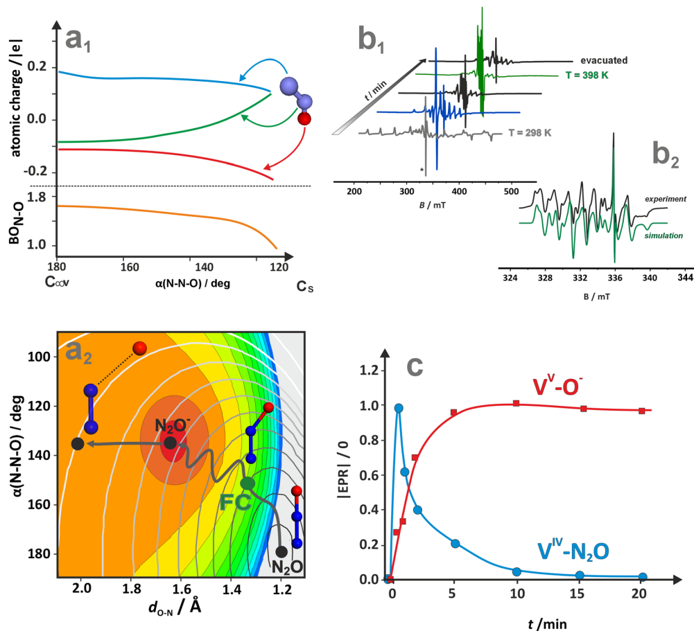
Fig. 40 Variation of the charge redistribution and the N–O bond order for the N 2 O molecule upon bending (a 1 ), and overlay of the molecular energy surfaces of N 2 O (grey iso-energy lines) and N 2 O - (colour coded areas) with the schematic reaction pathway leading from linear N 2 O molecule, through bent transition state at Frank–Condon (FC) locus into shallow minimum on the N 2 O - PES, prompting an eventual dissociation of the N 2 O - transient (a 2 ). Adapted from ref. 379 under the terms of the CC BY 4.0 license, Copyright 2024, published by the American Chemical Society. Evolution of the EPR spectra recorded during the reaction of N 2 O with VO 2 centres entrapped in BEA zeolite (b 1 ), together with simulation of the EPR signal due to [VO 2 + ]-O - species (b 2 ) (adapted from ref. 295 with permission from the Royal Society of Chemistry, Copyright 2016) together with the corresponding plot of gradual transformation of [VO 2 ]-N 2 O into [VO 2 + ]-O - via an electron transfer mechanism (c).
