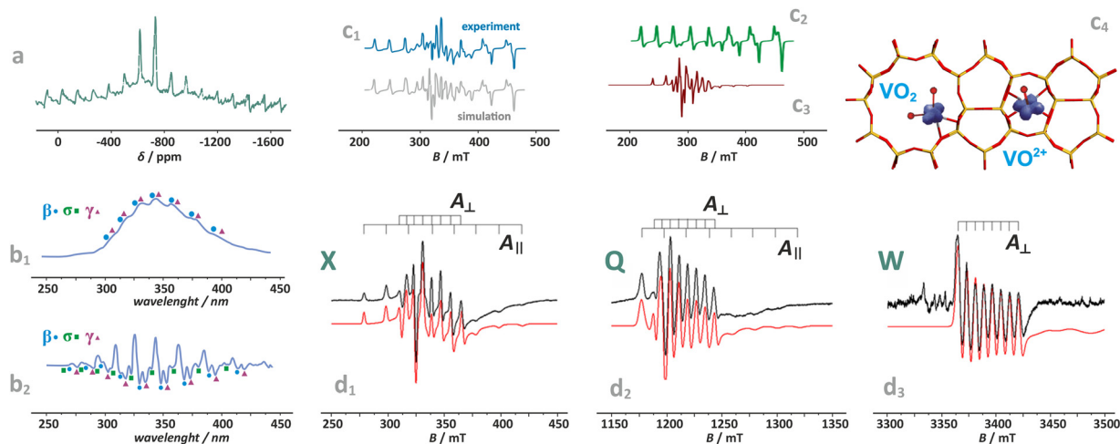
Fig. 9 Exemplary NMR (a) and photoluminescence spectra of vanadium(v)-oxo species in BEA zeolite (b 1 ) and (b 2 ), ( \beta , \sigma , \gamma indicate three vanadium species of various structures), based on data published in the ref. 130 redrawn and modified for clarity. Simulated and experimental EPR spectra of vanadium in the dealuminated BEA zeolite (c 1 ) and the component signals of VO^{2+} (c 2 ) and VO_2 (c 3 ) species, together with spin density contours calculated for the VO_2 and VO^{2+} species (c 4 ), adapted from ref. 110 with permission from American Chemical Society, Copyright 2007. Experimental (black) and simulated (red) EPR spectra of the VO^{2+} /ZSM-5 sample registered at (d 1 ) X-band, (d 2 ) Q-band, and (d 3 ) W-band, adapted from ref. 37 with permission from Elsevier Inc., Copyright 2020.
