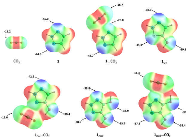
Fig. 3 MESP on the 0.005 a.u. isodensity surface for \text{CO}_2 , 1 , 1OH , 1OH 2 , and their \text{CO}_2 complexes. V_{\text{min}} values ( \text{kcal mol}^{-1} ) and \text{N}\cdots\text{C} , \text{O}\cdots\text{H}\cdots\text{O} distances ( \text{\AA} ) at the M06-2X/cc-pVQZ level of theory. Color gradient: blue (electron-rich) to red (electron-deficient).
