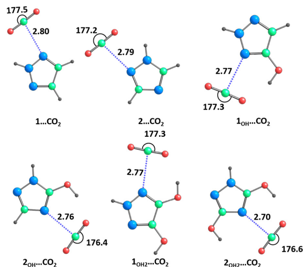
Fig. 4 Optimized geometries of the neutral triazole- \text{CO}_2 complexes computed at the M06-2X/cc-pVQZ level of theory. Bond lengths are in \text{\AA} and bond angles in degrees. Color key: gray – H, blue – N, green – C, red – O.
