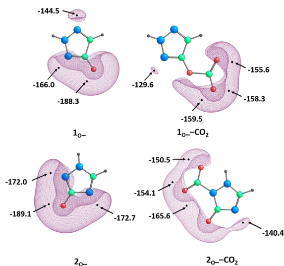
Fig. 5 MESP topography of anions 1O - , 2O - and their most stable \text{CO}_2 adducts computed at the M06-2X/cc-pVQZ level of theory. Black dots indicate V_{\text{min}} value in \text{kcal mol}^{-1} . Isosurface value: -125 \text{kcal mol}^{-1} . Color key: gray – H, blue – N, green – C, red – O.
