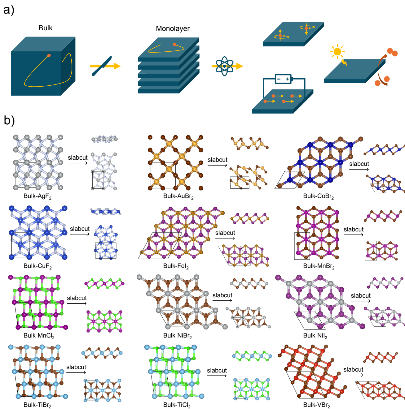
Fig. 1 Prediction of isolated 2D monolayers derived from bulk counterparts. (a) Monolayers slabcut from bulk structures and optimized through ab initio calculations, exhibiting distinct electronic, catalytic, and spintronic properties due to electron confinement effects. (b) Examples of optimized bulk and monolayer crystal structures, with spheres representing different elements: Ag (gray), Au (gold), Br (brown), Cl (fluorescent green), Co (dark blue), Cu (blue), F (light blue), Fe (dark yellow), I (dark purple), Mn (light purple), Ni (silver), Ti (aqua blue), and V (red). Bulk structures visualized from a top view while monolayers consisting of a side view and a top view.
