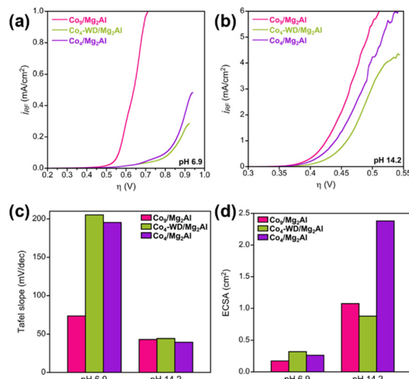
Fig. 3 OER activity of the nanocomposites. LSV polarization curves using (a) 0.1 M NaP i buffer with 1 M \text{NaNO}_3 as an electrolyte at pH 6.9 and (b) 1 M KOH electrolyte at pH 14.2. (c) Extracted Tafel slopes. (d) Estimated ECSA values.
