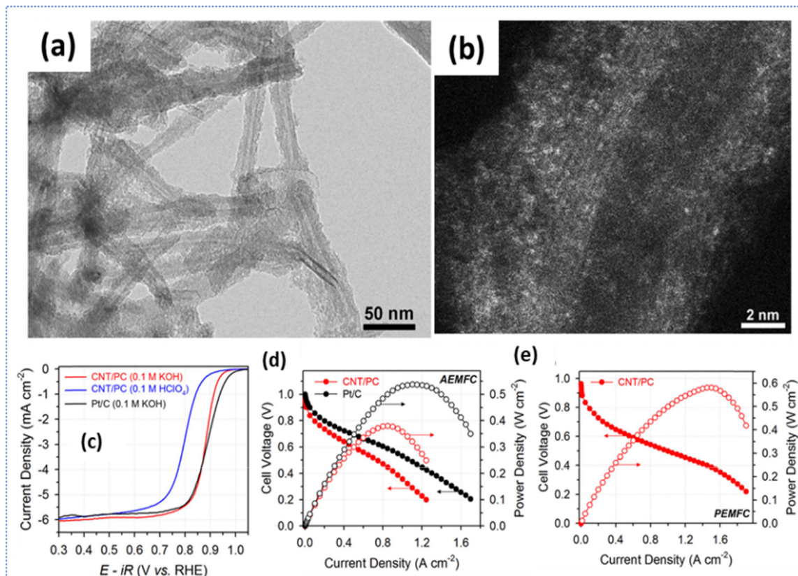
Fig. 6 (a) TEM and (b) HAADF-STEM images of CNT/PC. (c) ORR activity of CNT/PC. (d) AEMFC performances using the CNT/PC and Pt/C catalysts, and (e) PEMFC performance with the CNT/PC cathode catalyst. Reproduced from ref. 111 with the permission from the American Chemical Society, copyright 2016.
