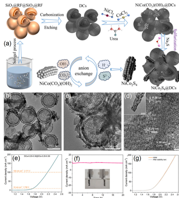
Fig. 14 (a) Schematic illustration of the synthesis of \text{NiCo}_2\text{S}_4 @DCs. (b)–(d) TEM data of the composite system. (e) LSV curve of the composites recorded in 1 M KOH. (f) Chronoamperometry measurement at 1.736 V for 20 h in 1 M KOH; the inset depicts the two-electrode operating configuration. (g) LSV data collected before/after the chronoamperometry test. Reproduced with permission from ref. 96. Copyright 2024 Elsevier.
