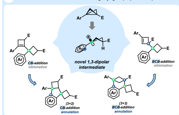
Scheme 1. A) Bioisosteres derived from reactions involving BCBs. B) Lewis acid catalysed BCB reactivity: 1,3-dipolar cycloaddition and 1,2-addition with cyclobutene formation. C) This work: BCB dimerisation.
