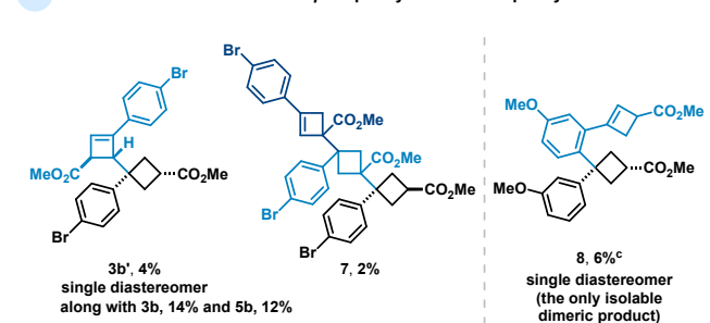
Scheme 2. (A) Major dimerisation pathways found and (B) minor dimerisation pathways observed in the reactions of p -Br-phenyl- and m -OMe-phenyl-substituted BCBs ( 1b , 1c ) a One drop (~50 \mu L) of H 2 SO 4 per 1 mL of solvent is used. b Reactions conditions: BCB (0.3 mmol), Sc(OTf) 3 (20 mol%), CH 2 Cl 2 , 24 h, 25 °C. c 30% of corresponding cyclobutene 2c .
