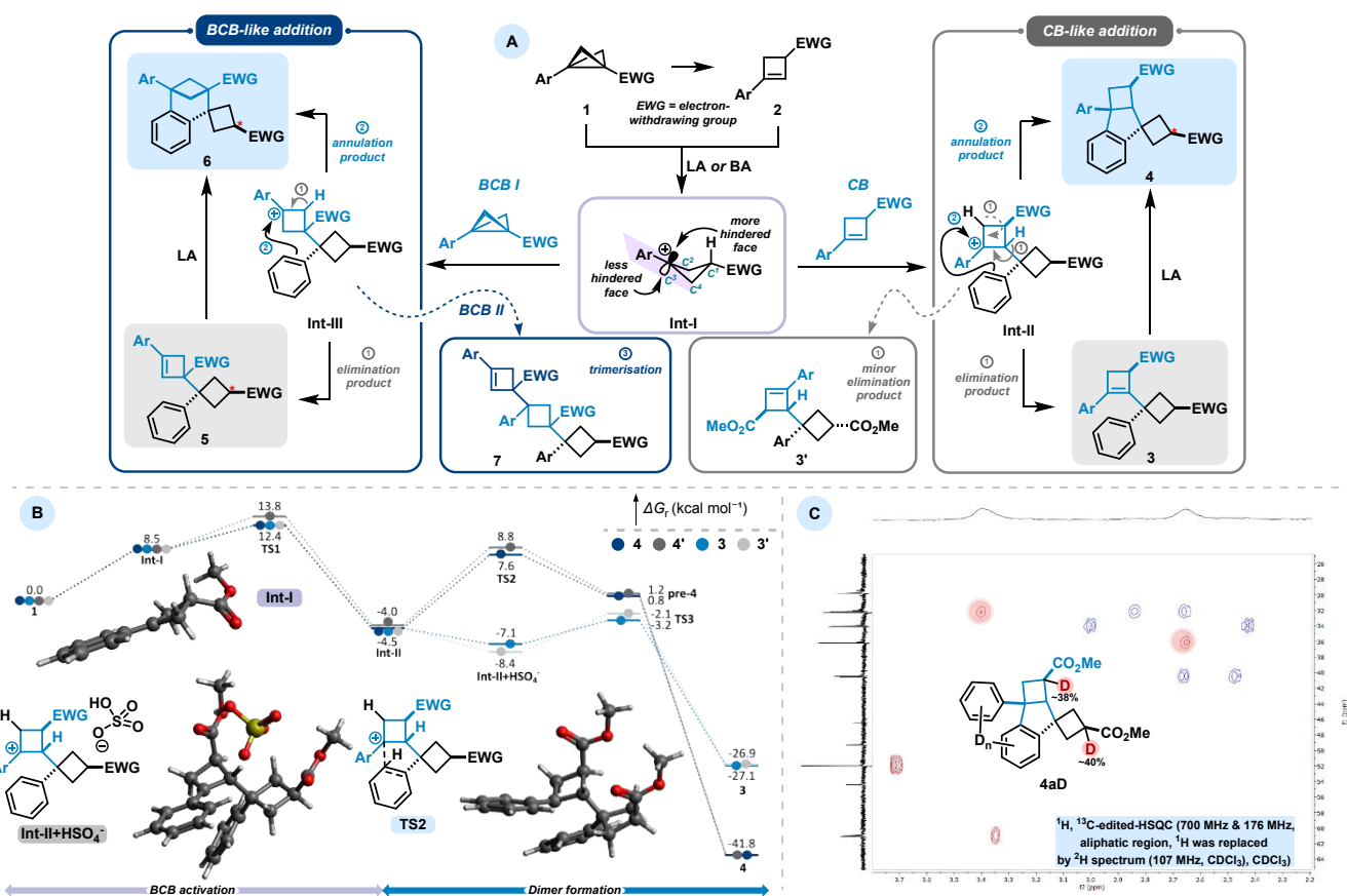
Scheme 3. (A) Proposed mechanism of observed dimerisation pathways. (B) Energy diagram of the DFT studies (M06-2X/def2-TZVP-D3//r 2 scan-3c, CPCM (CH 2 Cl 2 )). (C) 1 H, 13 C-edited-HSQC (700 MHz & 176 MHz, zoomed aliphatic region, 1 H was replaced by 2 H spectrum (107 MHz, CDCl 3 , CDCl 3 ). Scaffold 4 synthesised in D 2 SO 4 . BCB 1a (0.3 mmol), D 2 SO 4 99,5 atom% D, CH 2 Cl 2 , 25 °C, 24 h
