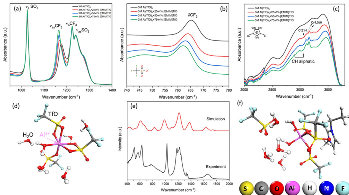
Fig. 10 FT-IR spectra of AlTfO at each concentrations of EMIMTfO. (a) 900 and 1400 \text{cm}^{-1} . (b) 740 and 780 \text{cm}^{-1} . (c) 2000 and 4000 \text{cm}^{-1} . (d) Al(TfO) 3 ·6H 2 O Geometries with all the TfO - ions are being bi-coordinated to the Al 3+ ion. (e) Comparison of experimental and simulated IR spectra of AlTfO in water. (f) Relaxed geometries of Al(TfO) 3 ·6H 2 O with EMIMTfO.
