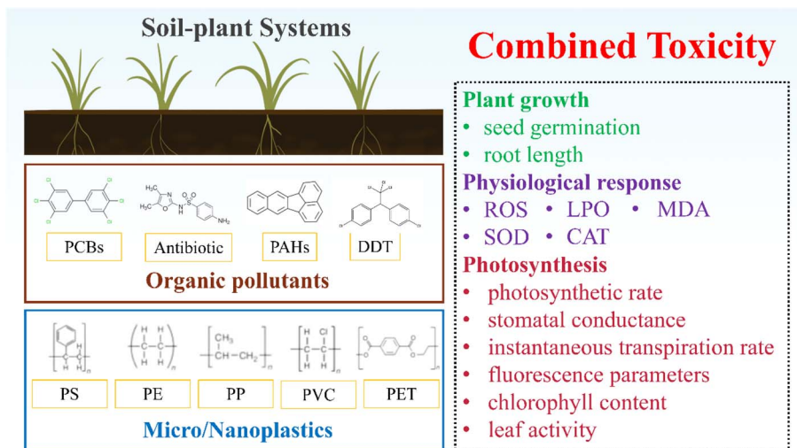
Fig. 3 Ecotoxicological implications of MNPs and OPs interactions in soil–plant systems.
