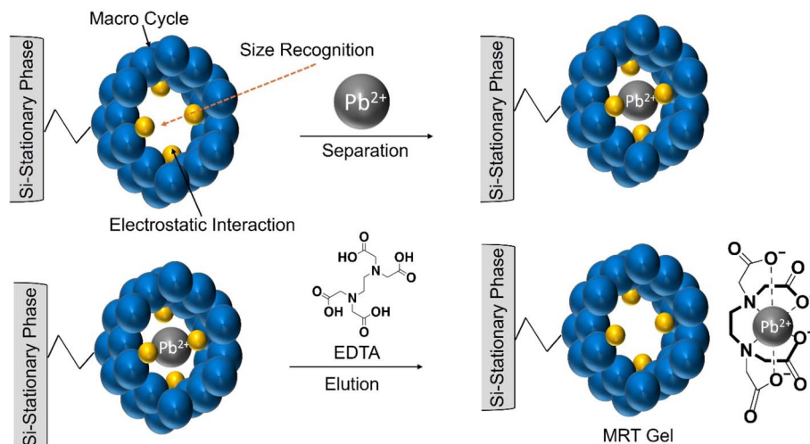
Fig. 9 A schematic illustration of the selective separation of Pb^{2+} by AnaLig Pb-02 MRT-SPE system.
