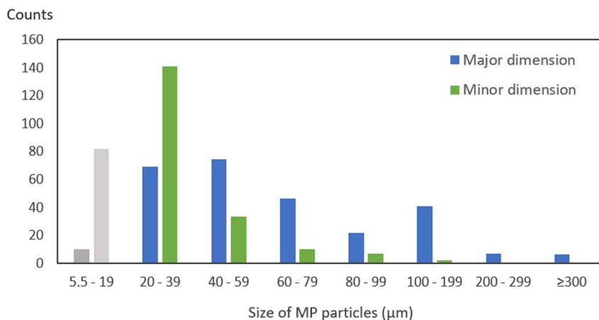
Fig. 4 Size distribution of MPs identified in wastewater samples from Sisimiut. The figure indicates counts of particles within each size group per liter sample. The size distribution is shown for the dimensions of the particles measured on the longest and the shortest edge, i.e. major and minor dimensions, respectively, by \mu\text{FTIR} image analysis and use of siMPLe software ( https://simpleplastics.eu/ ) data output. Note: the size group of 5.5–19 \mu\text{m} (grey colors) is below the filter used in the extraction procedures, wherefore the number must be seen as an absolute minimum.
