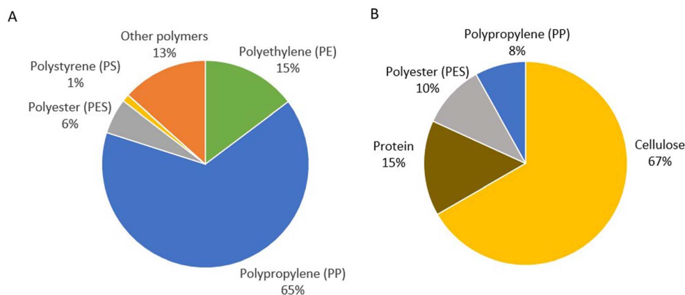
Fig. 3 Polymer distribution of (A) all MPs (20–1000 \mu\text{m} ) and (B) fibers only, in wastewater samples from Sisimiut identified by \mu\text{FTIR} analysis.
