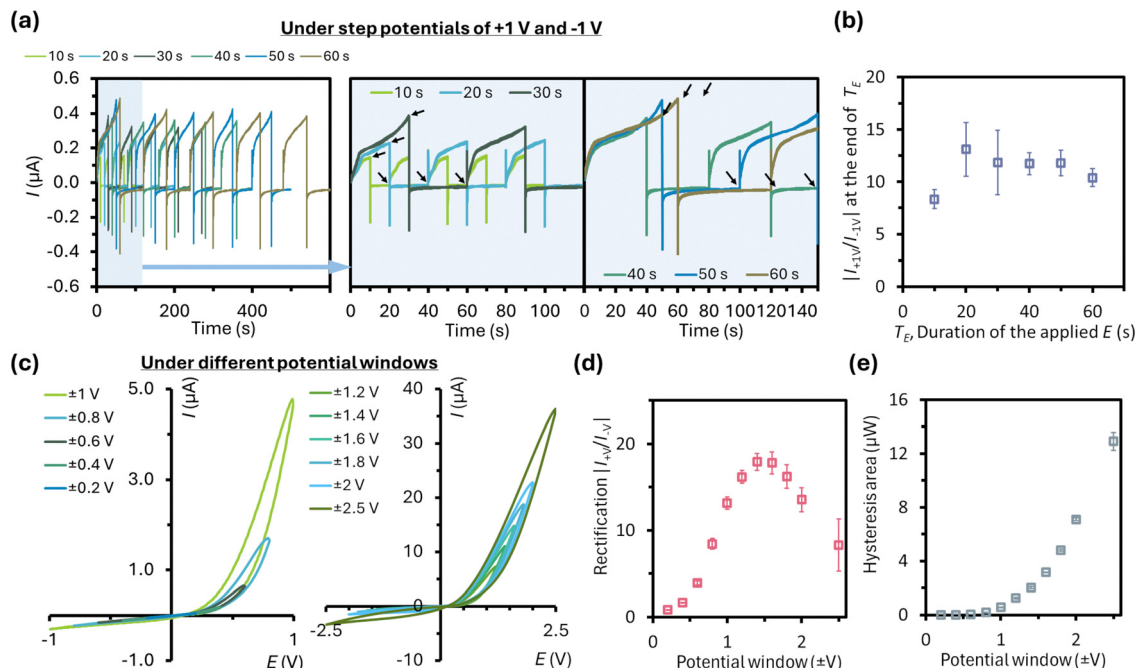
Fig. 4 (a) I - t plots of the bipolar electrochemical memristor under chronoamperometry step potentials of \pm 1 V and \pm 1 V with step durations ( T_E ) of 10 s to 60 s and the magnified plots. Black arrows indicate the data taken for calculating |I_{+1V}/I_{-1V}| . (b) Plot of |I_{+1V}/I_{-1V}| against T_E (0.5 mM \text{Na}_2\text{SO}_4 , 10-nm PCTE). (c) I - V plots under potential windows of \pm 0.2 V to \pm 1 V and \pm 1.2 V to \pm 2.5 V and (d) the corresponding |I_{+1V}/I_{-1V}| and (e) area of the hysteresis loop against the potential window (0.5 mM \text{Na}_2\text{SO}_4 , 0.04 \text{ V s}^{-1} , 10-nm PCTE).
