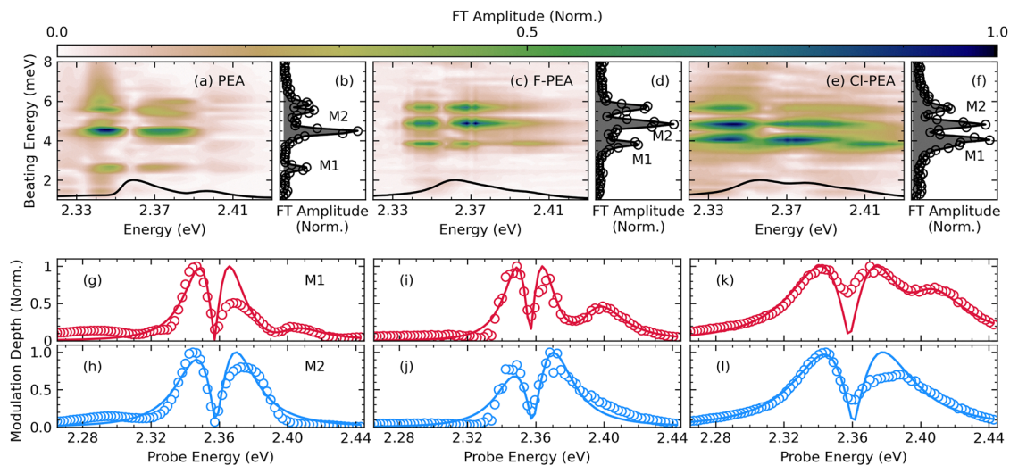
Fig. 4 Linear absorption (black line) and beating spectra as a function of detection energies for (a) (PEA) 2 PbI 4 , (c) (F-PEA) 2 PbI 4 , and (e) (Cl-PEA) 2 PbI 4 . Probe-energy-integrated vibrational spectra for (b) (PEA) 2 PbI 4 , (d) (F-PEA) 2 PbI 4 , (f) (Cl-PEA) 2 PbI 4 respectively. All measurements were taken at 15 K. The corresponding spectral cuts of RISRS beating map and fitting results using eqn (2) and (3). This figure shows the modulation depth for phonon mode 1 (M1) and phonon mode 2 (M2), where spectral cuts were taken at (g) 2.3–2.9 meV and (h) 4.1–4.8 meV for (PEA) 2 PbI 4 , (i) 3.6–4.1 meV and (j) 4.5–5.3 meV for (F-PEA) 2 PbI 4 , (k) 3.6–4.4 meV and (l) 4.6–5.2 meV (Cl-PEA) 2 PbI 4 . The data is represented with open circles and the fit is the solid line.
