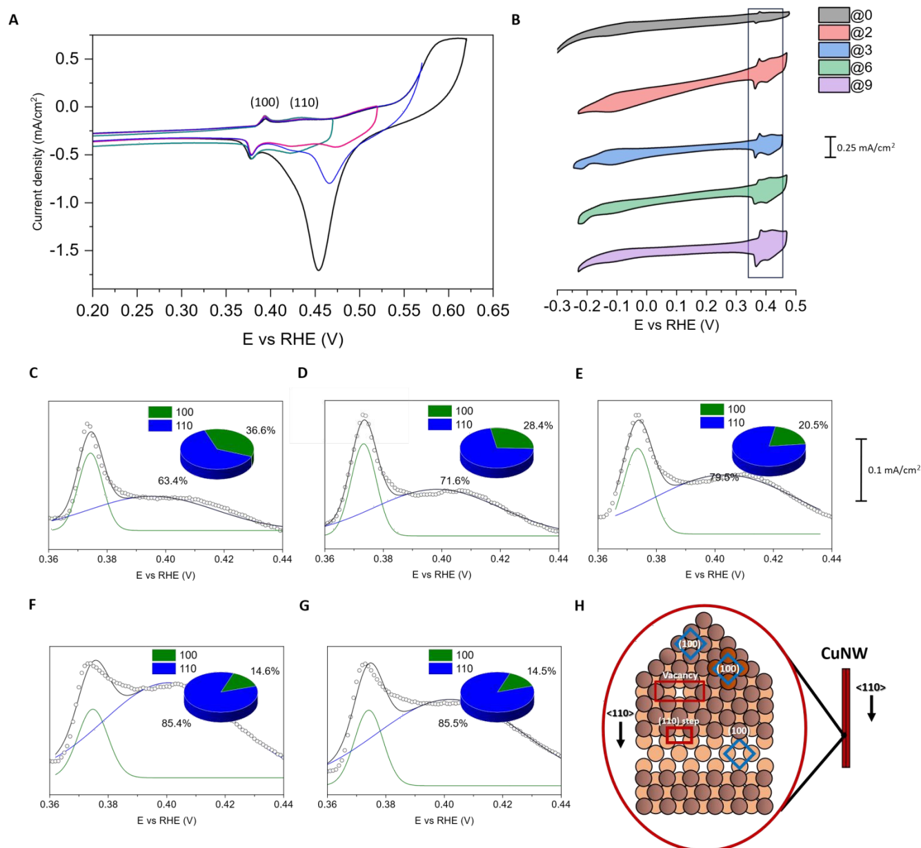
Fig. 4. A) Cyclic voltammetry of CuNWs@3 recorded in 1M NaOH, in a three-electrode cell configuration under Ar saturated solution, inverting at different stage the oxidation potential: +0.47 V (green), +0.52 V (magenta), +0.57 V (blue), +0.62 V (black). B) Cyclic voltammeteries were recorded in 1M NaOH, in a three-electrode cell configuration under Ar saturated solution and atmosphere. The black rectangle represents the magnification region. C)-G) Zoom of CV for CuNWs@0 (C), CuNWs@2 (D), CuNWs@3 (E), CuNWs@6 (F), CuNWs@9 (G) in 1M NaOH. The dotted curves represent the experiment CV's signals, and the black curves the simulated one. The red and blue curves represent the deconvoluted peaks of (100) and (110) peaks respectively. H) Representation of crystal step (110) on the (100) surface of CuNW. The dark Cu elements are the first atomic layer of the surface, the lighter represents the second atomic layer, and the dark orange the possible defectiveness.
