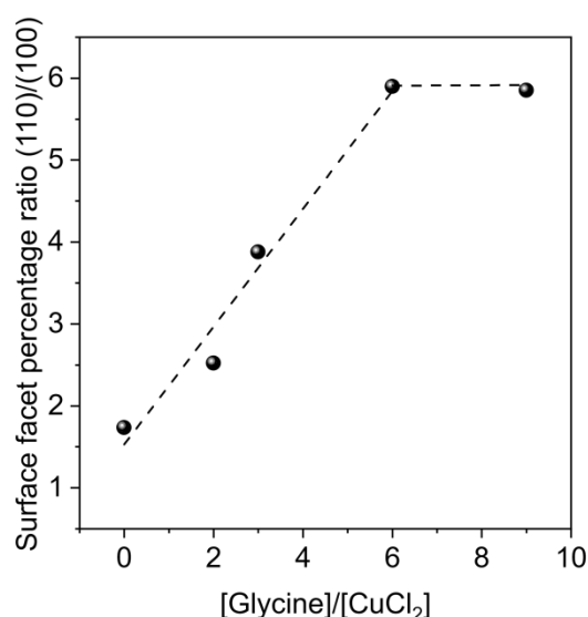
Fig. 5. Dependence of surface facet ratio on the quantity of glycine used in the synthesis protocol.
