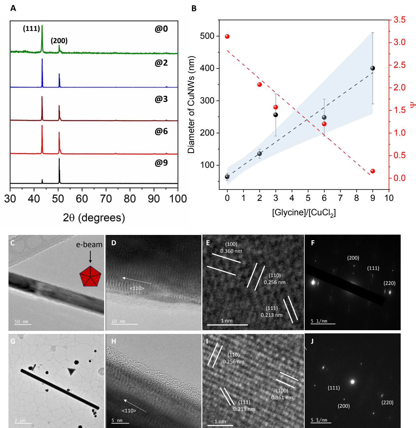
Fig. 2. A) XRD patterns of CuNWs synthesized with different quantities of glycine: 0 eq (green), 2 eq. (blue), 3 eq. (dark red), 6 eq. (red), 9 eq. (black). B) Plot of the dependence of average diameter of CuNWs (black dots) and of \psi (red dots) on the equivalents of glycine used in the synthesis. Error bars for diameters in black and 95% confidence bands are in light blue. C) TEM image of CuNWs@0. D) HR-TEM image of CuNWs@0. E) HR-TEM details of crystal lattice of CuNWs@0. F) SAED of single CuNWs@0. G) TEM image of CuNWs@9. H) HR-TEM image of CuNWs@9. I) HR-TEM details of crystal lattice of CuNWs@9. J) SAED of single CuNWs@9.
