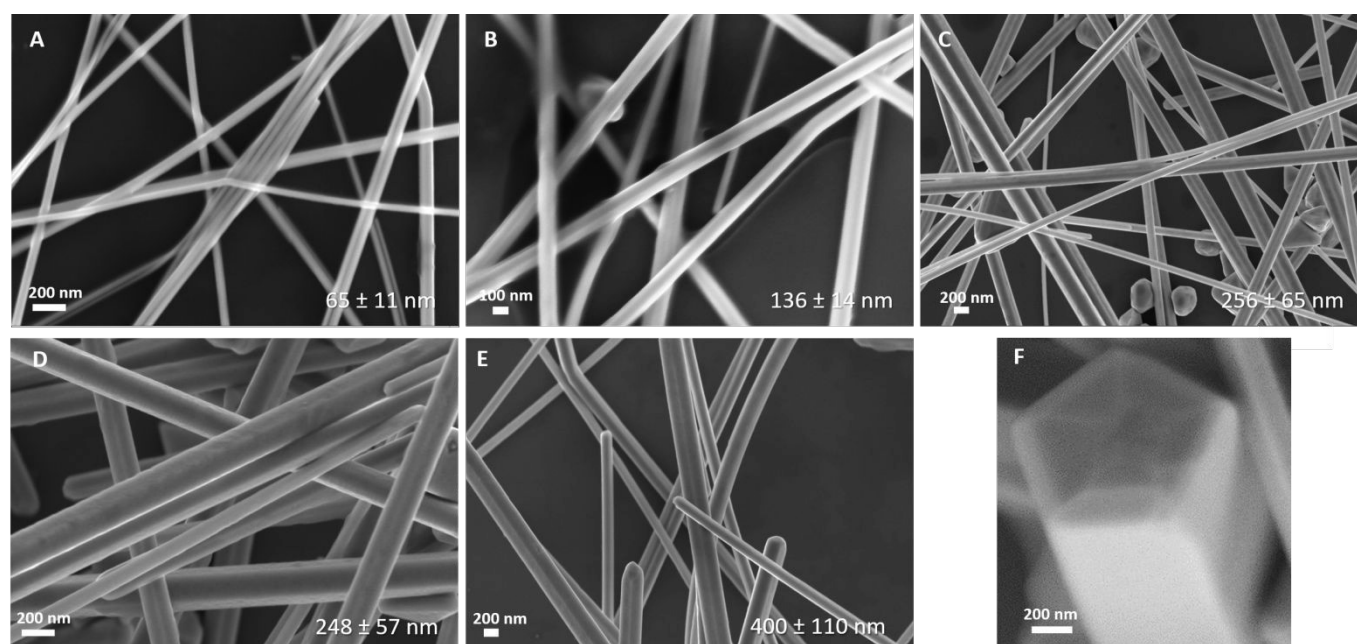
Fig 1. SEM images of CuNWs synthesized employing different quantities of glycine. A) 0 eq. B) 2 eq. C) 3 eq. D) 6 eq. E) 9 eq of glycine. F) Detail of CuNWs@9 tail highlighting the penta-twinned nature of the CuNWs. The average diameter of CuNWs is highlighted on the bottom of each image.
