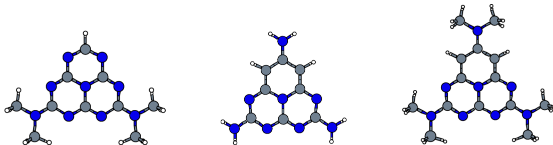
Fig. 5 Molecules presenting a \Delta E_{\text{ST}} < 0 value with the largest calculated f_{\text{osc}} values.
