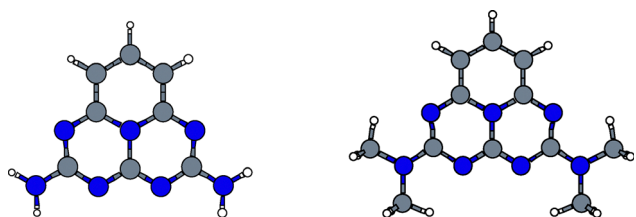
Fig. 6 Molecules presenting a \Delta E_{\text{ST}} > 0 value with the largest calculated f_{\text{osc}} values.
