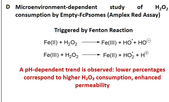
Fig. 2 Trapping of radicals at different pH with DMPO formed by the Fenton reaction of FcPsomes in the presence of hydrogen peroxide as a proof of concept. (A) The 1 : 2 : 2 : 1 intensity pattern and a hyperfine line splitting of about 14.9 G is characteristic for the DMPO adduct formed by trapping the OH radical from the Fenton reaction by using FcPsomes A at different pH values. (B) Three replicates taking the maximum intensity of second line of the signal of spin adduct for mixtures of FcBCP A, \text{H}_2\text{O}_2 and DMPO at different pH values. (C) the maximum intensity of the second line for spin-trapping experiments with FcBCP, FcPsomes A, C or D. Fe content determined by ICP-OES in 1 \text{ mg mL}^{-1} solution of FcPsomes: 9.8 of \text{Fe } \mu\text{g mL}^{-1} in FcPsomes A, 12.4 of \text{Fe } \mu\text{g mL}^{-1} in FcPsomes C and 3.3 of \text{Fe } \mu\text{g mL}^{-1} in FcPsomes D. Conditions in all samples: 0.21 mM of ferrocene containing in 10 mM NaCl at different pH values. (D) Microenvironment-dependent study of hydrogen peroxide consumption by FcPsomes using Amplex Red assay (fluorometric measurements). It is an indirect method: the lower the fluorescence of resorufin, obtained from converted Amplex Red by myoglobin, the more active the FcPsomes are.
