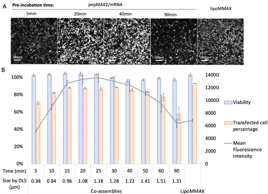
Fig. 4 Transfection efficacy of pepMAX2/mRNA pre-incubated in 250 mM NaCl solution for different time intervals. The N/P ratio was kept the same at 4, with the peptide concentration at 2 \mu M for 80 ng loading. The transfection efficiency was observed by (A) fluorescence microscope and quantified by (B) flow cytometry, with cell viability, percentage of cells transfected and mean fluorescence intensity (MFI) of the positive cells. LipoMMAX served as a control with the same mRNA loading as 80 ng/100 \mu L in the co-assemblies (data shown are mean \pm SD, n \geq 3 ).
